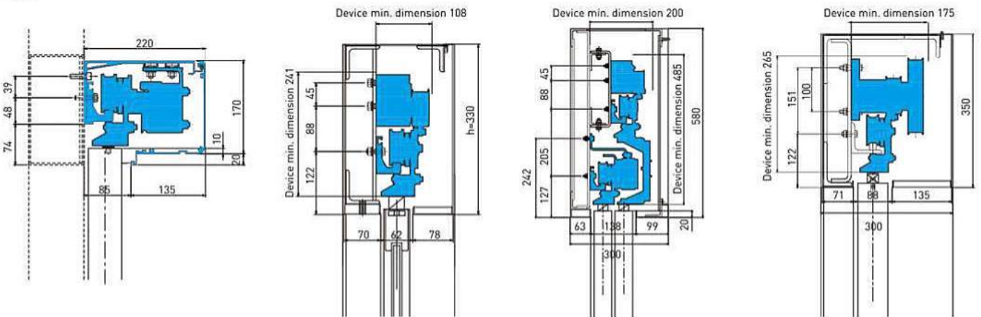
Other External-mounted Devices Frame VS-250SL-M View
